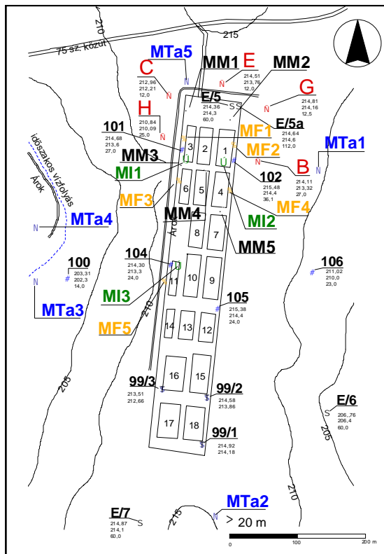
Fig.1. Scheme of the site
