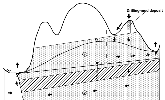
Fig.3. GW flow regime at the site
