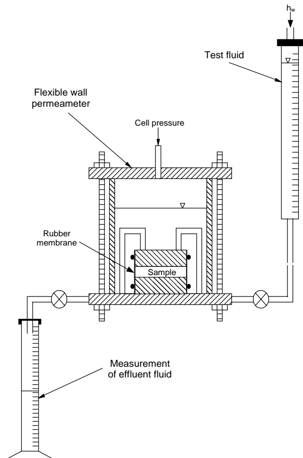
Fig.5 The measuring device
