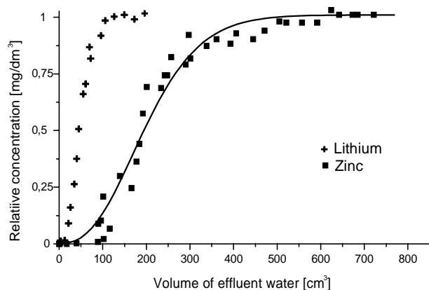
Fig 6. Break-through curves measured
