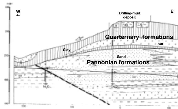
Fig.2. Representative cross section of the site
