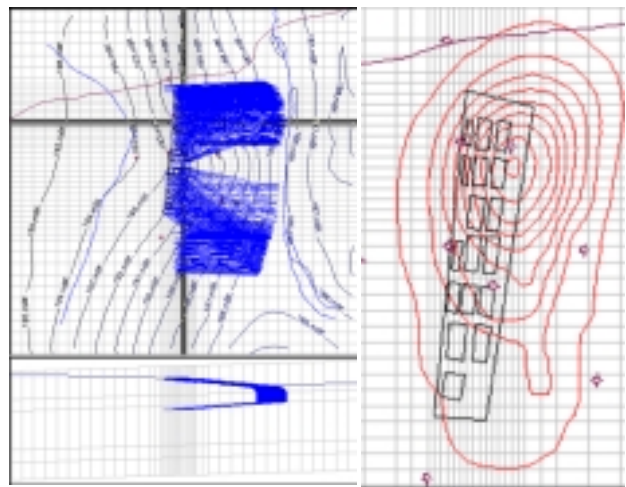
Fig.7. Pathlines starting from the deposit and concentration isochrones during natural attenuation
