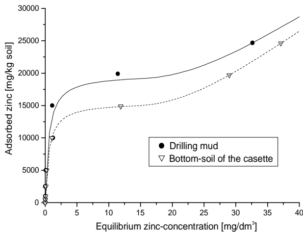
Fig.4. Adsorption isotherms of mud and soil
